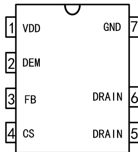
DIP7 Package
